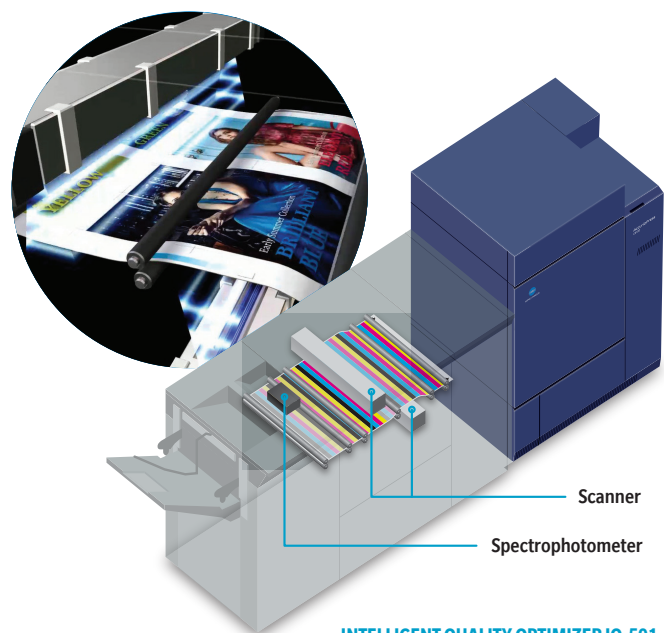
INTELLIGENT QUALITY OPTIMIZER IQ-501
